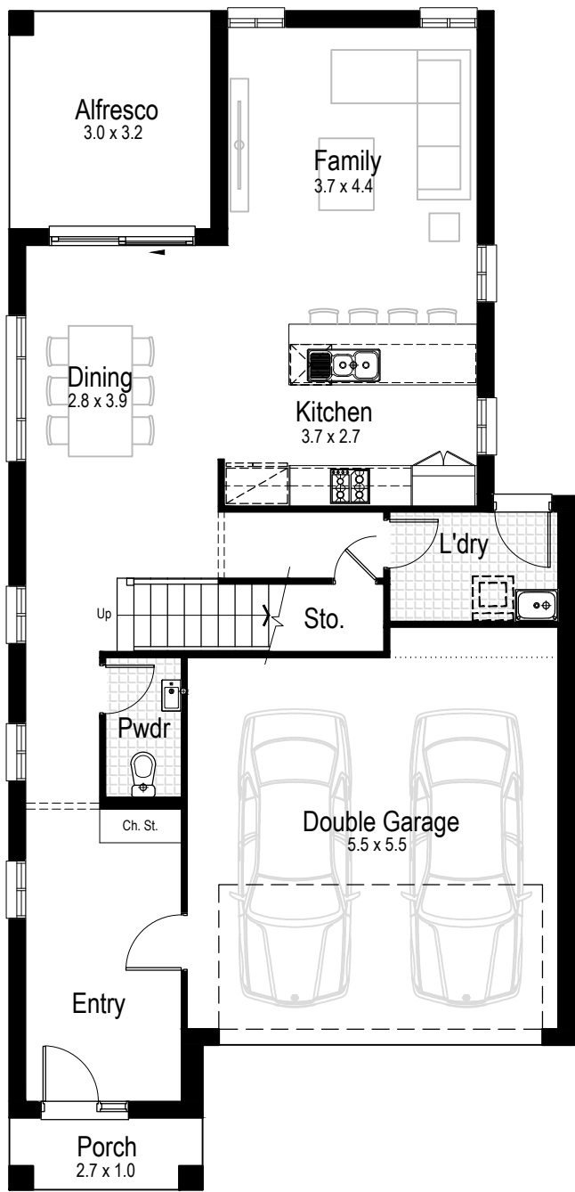
Ground Floor
